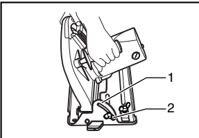
1. Bevel scale plate 2. Clamping screw
