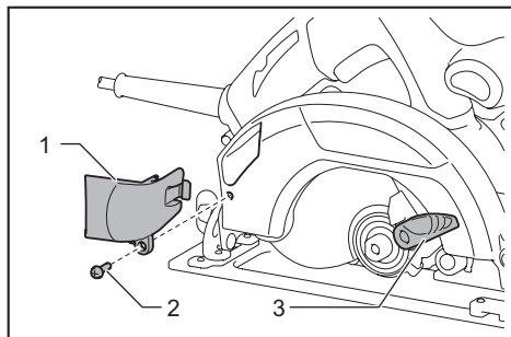
► 1. Dust nozzle 2. Screw 3. Lever (supplied with the dust nozzle)
