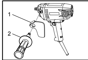
1. Cover 2. Side grip
