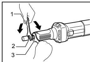
1. Wrench 13 2. Collet nut 3. Wrench 13
